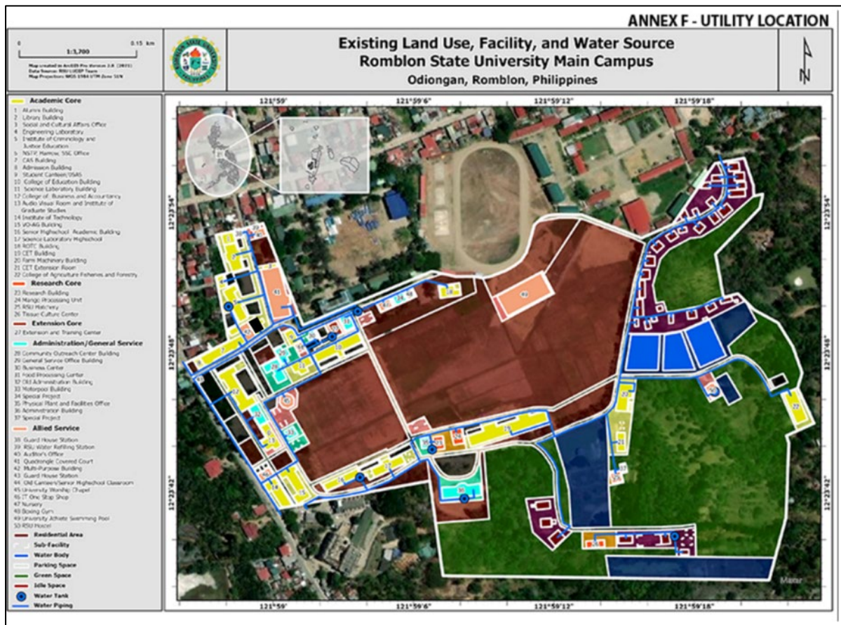
Figure: Existing Water Source of Romblon State University - Main Campus Source: Planning and Development Office
