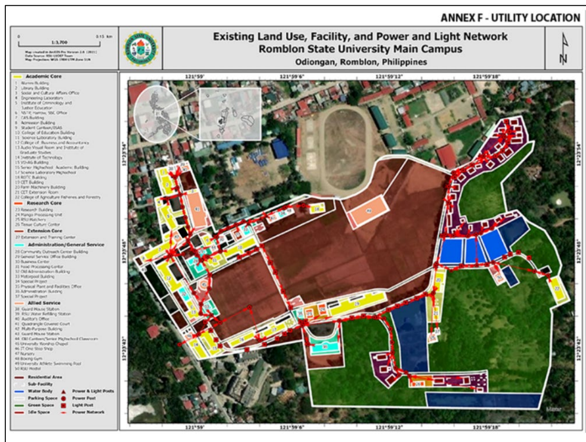
Figure: Existing Power and Lighting Network of Romblon State University - Main Campus
