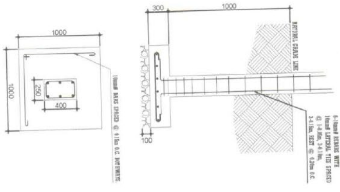
1 S-1 C-1-F1 DET PLAN SCALE 1:30
