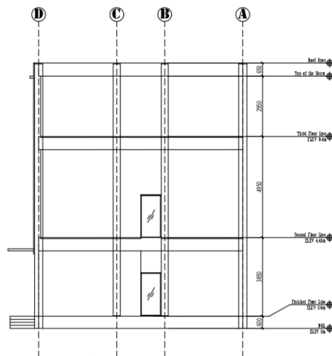
A-6 REAR ELEVATION SCALE 1:100
