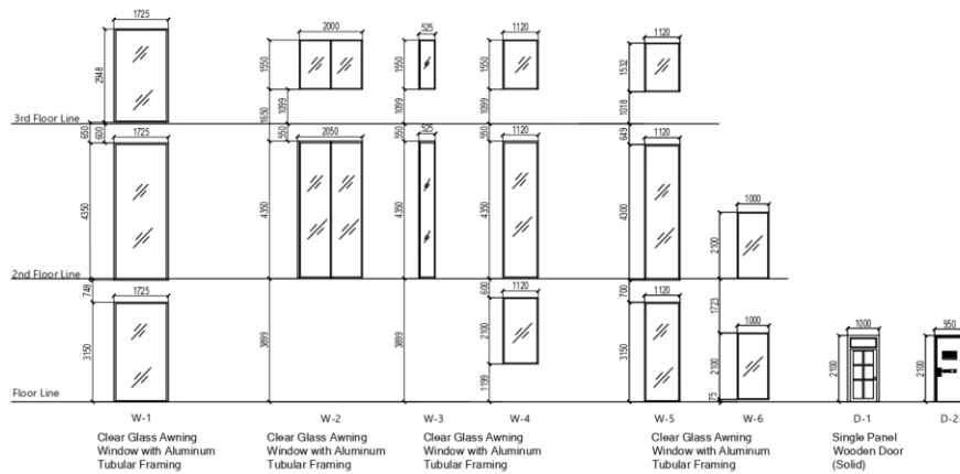
A-4 SCHEDULE OF DOORS AND WINDOWS SCALE 1:100
