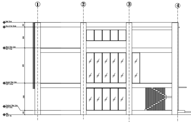
A-7 LEFT SIDE ELEVATION SCALE 1:100
