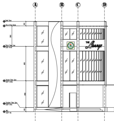
A-5 FRONT ELEVATION SCALE 1:100
