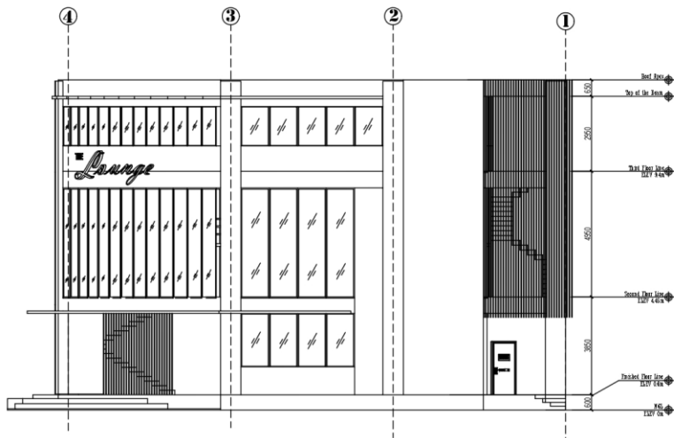
A-8 RIGHT SIDE ELEVATION SCALE 1:100
