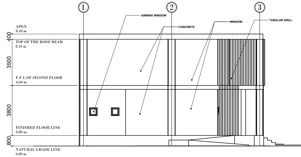
A 3 LEFT ELEVATION SCALE: _____ NTS
