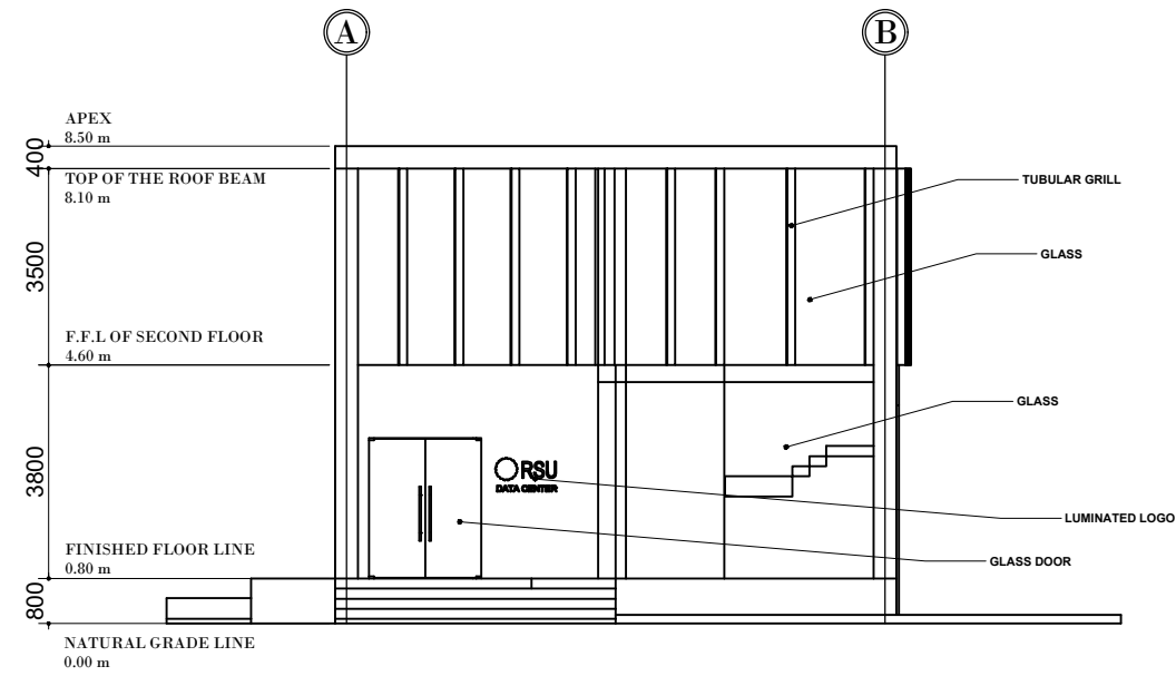
A 1 FRONT ELEVATION SCALE: _____ NTS
