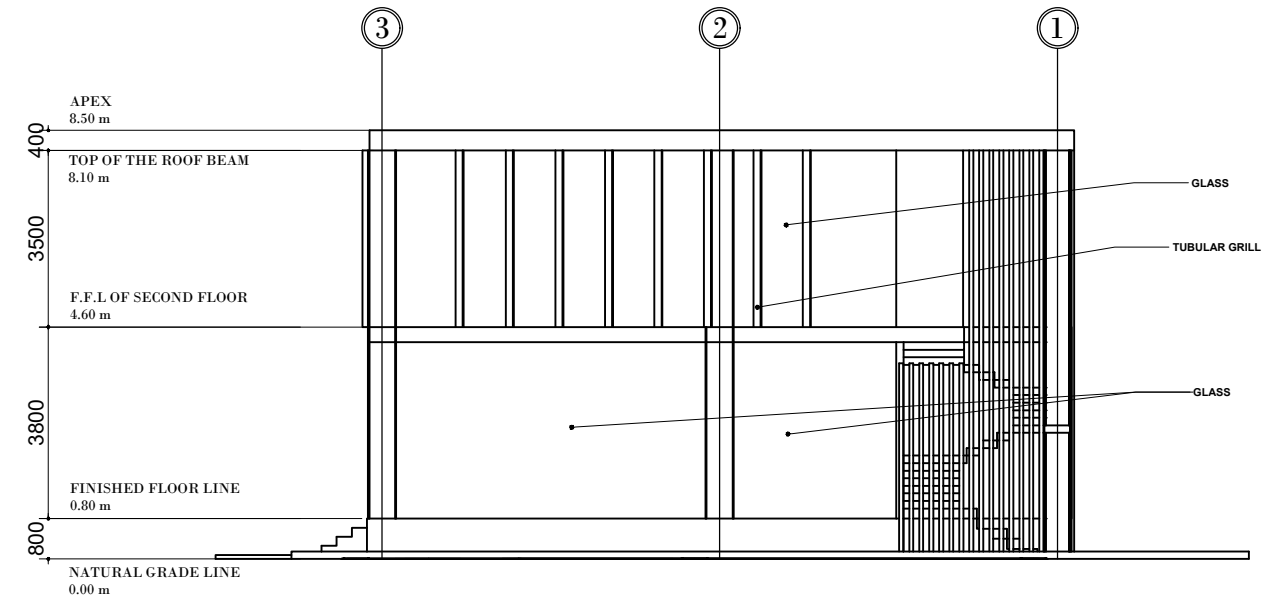
A 4 RIGHT ELEVATION SCALE: _____ NTS
