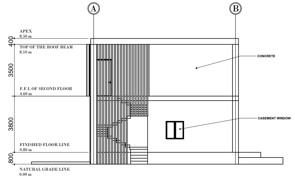
A 2 REAR ELEVATION SCALE: _____ NTS
