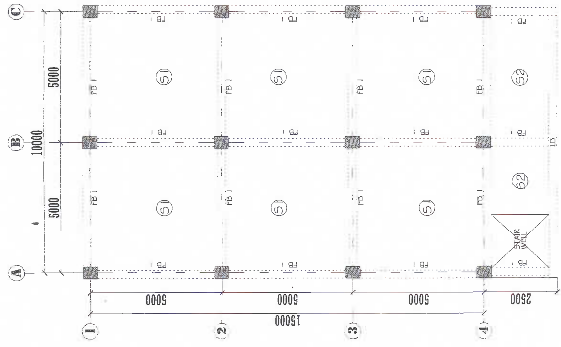
1 THIRD FLOOR FRAMING PLAN $-7 S-7 SCALE 1:100
