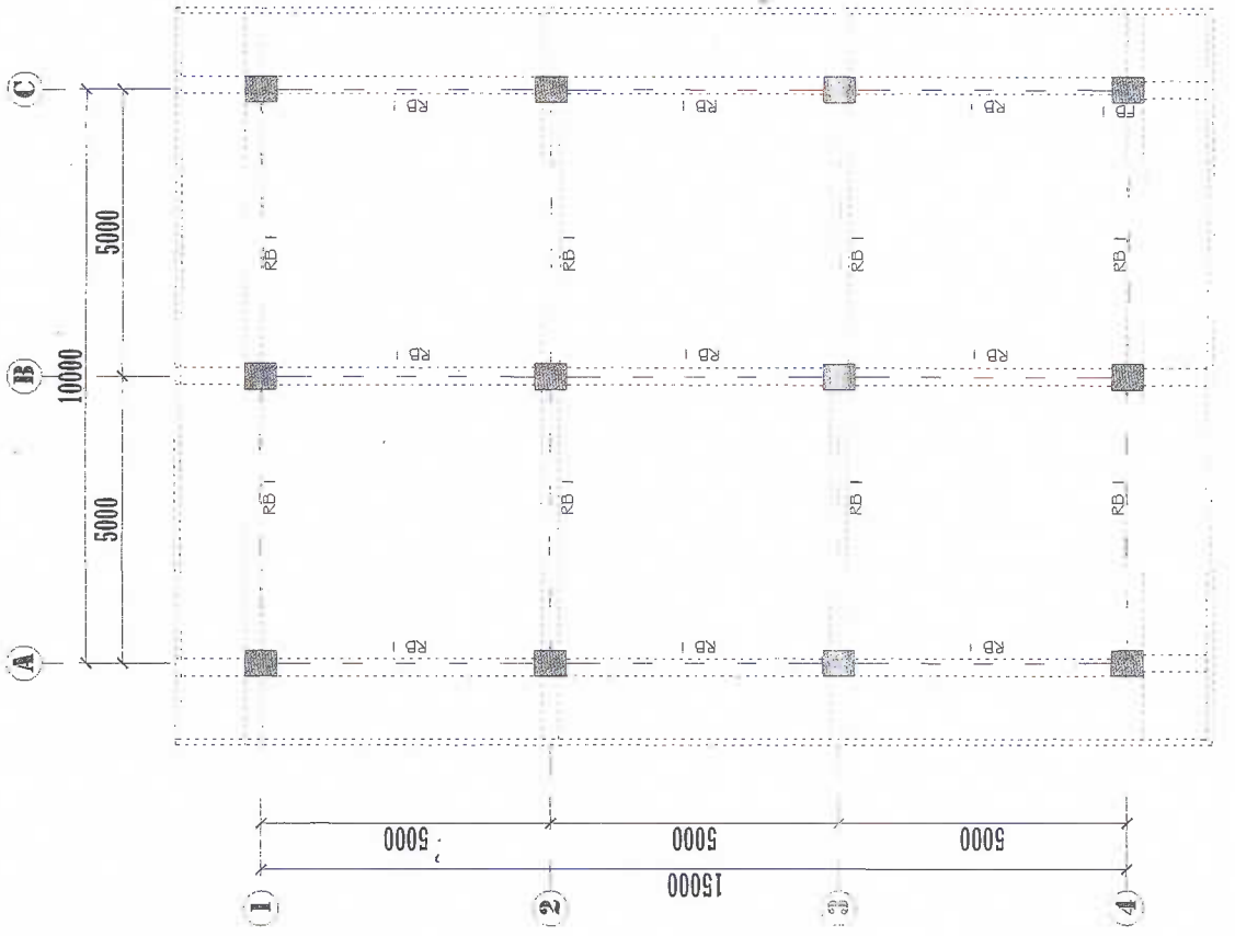
2 ROOF BEAM FRAMING PLAN $-7 S-7 SCALE 1:100
