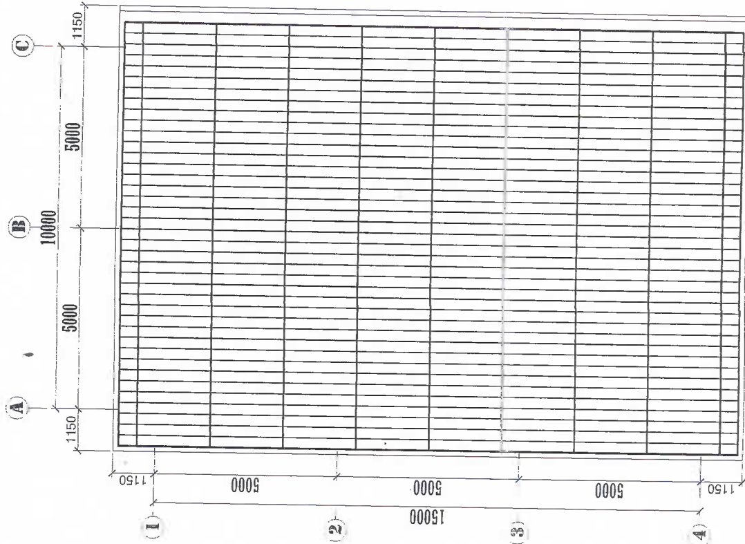
1 ROOF TRUSS FRAMING PLAN S-8S-8 SCALE 1:100
