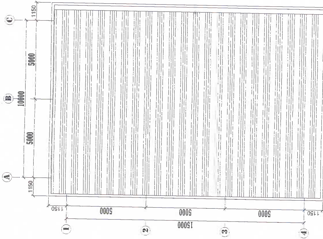
2 ROOF PLAN VIEW S-8S-8 SCALE 1:100
