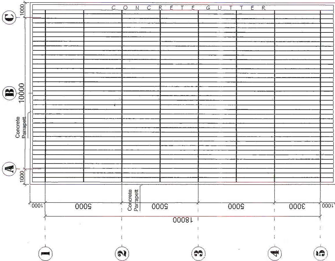
I ROOF TRUSS FRAMING PLAN 3:1000
