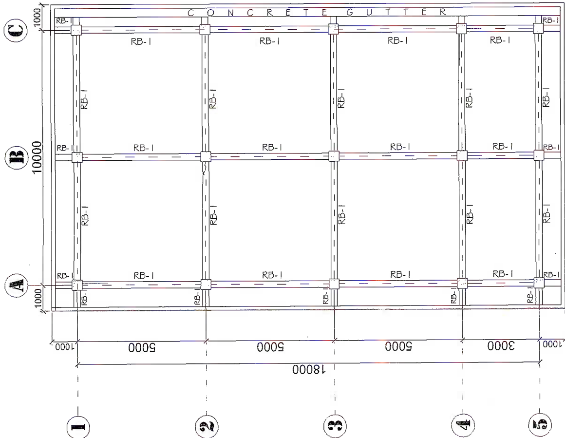
1 ROOF BEAM FRAMING PLAN 1:100 S-8
