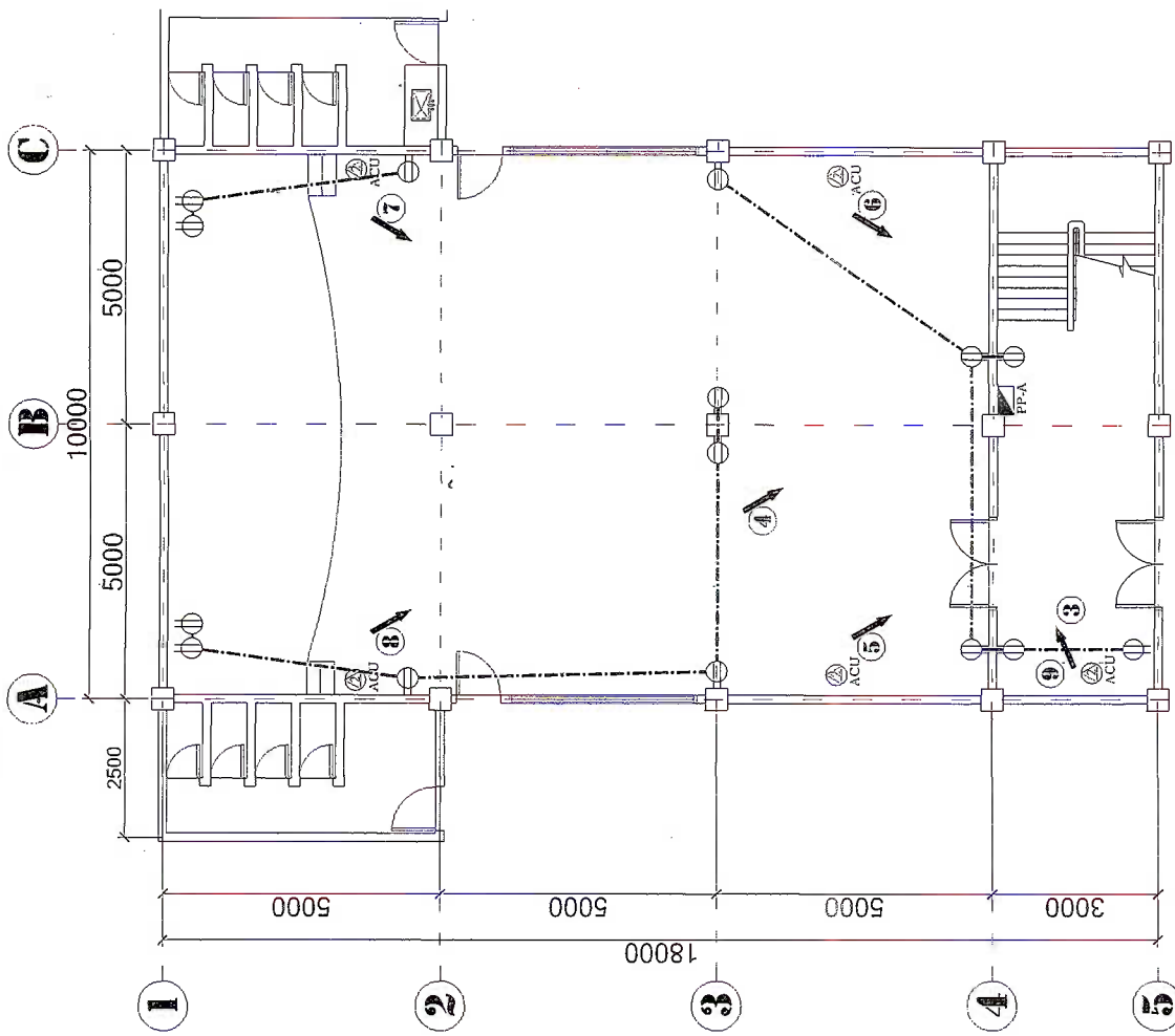
1 GROUND FLOOR C. O. LAYOUT PLAN E-2-E-2, SCALE 1:100
