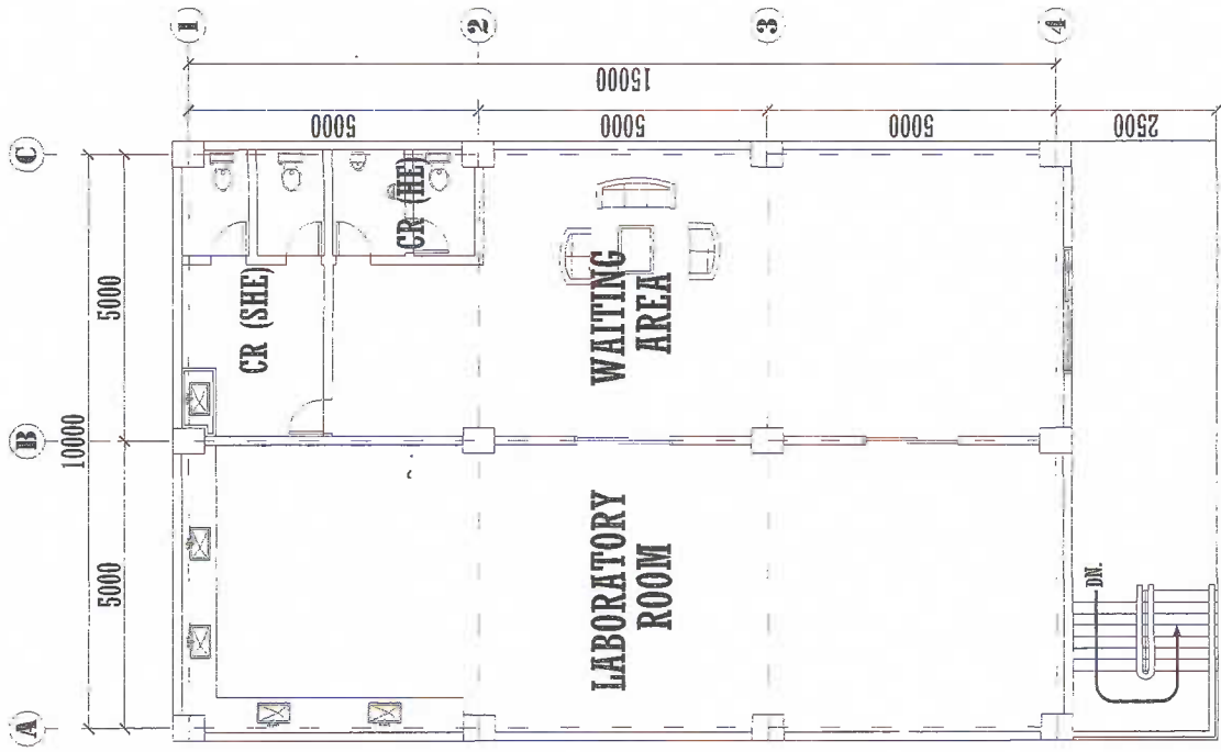
1 THIRD FLOOR PLAN A-3A-3 SCALE 1:100
