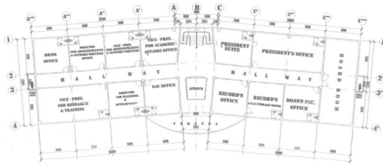
1 2ND FLOOR PLAN SCALE 1/3200
