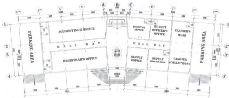
1 GROUND FLOOR PLAN SCALE 1/3200
